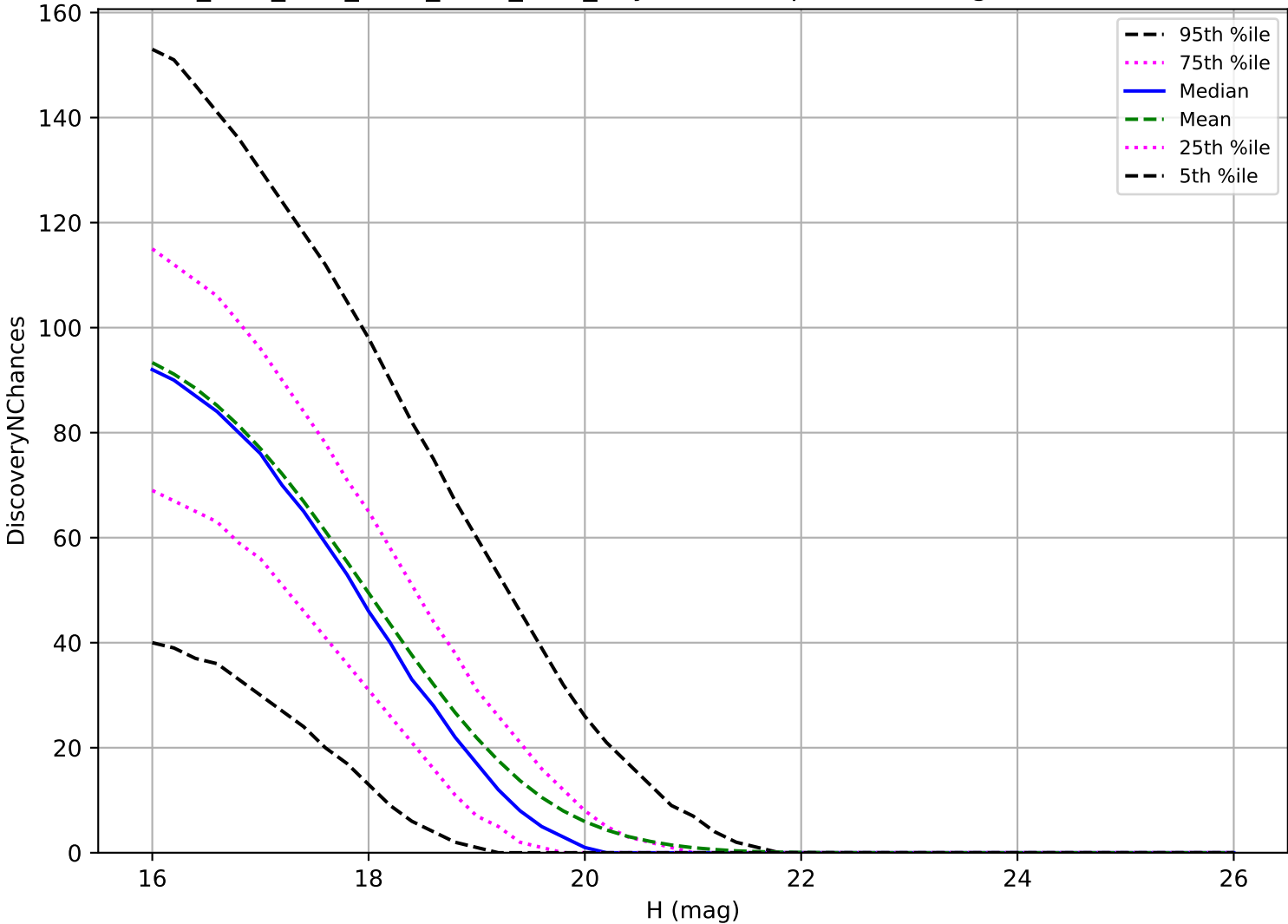
ddf_acor_sf15_lsf30_lsr20_v3.4_10yrs: MBA 3 pairs in 15 nights detection loss
