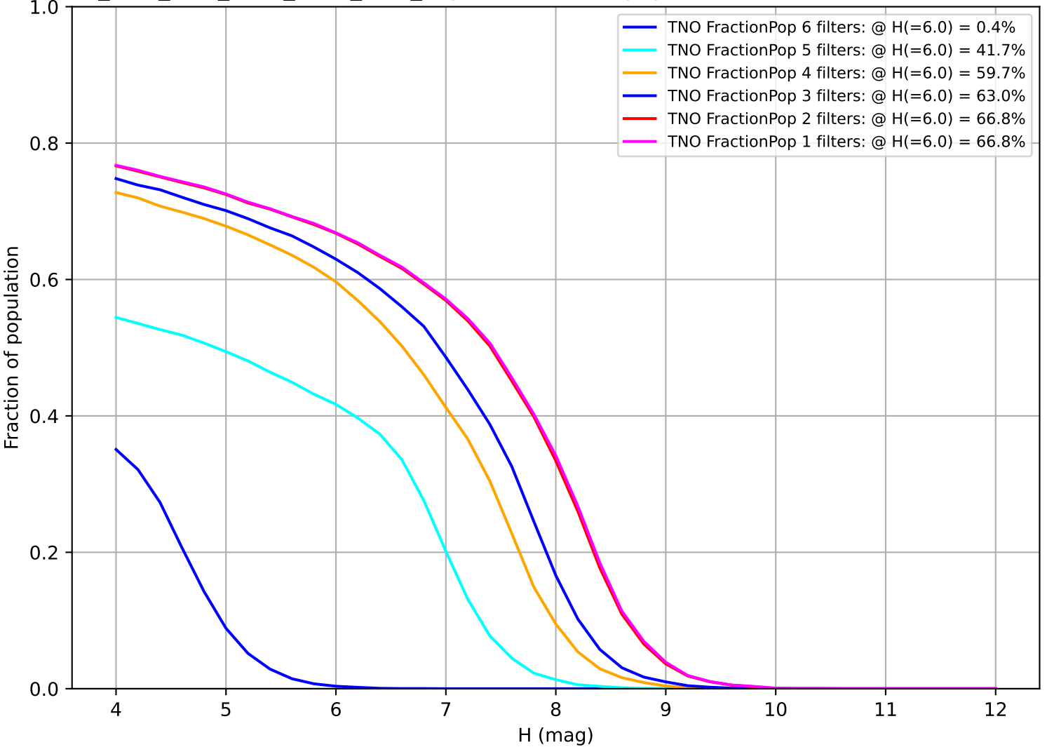
ddf_acor_sf15_lsf30_lsr20_v3.4_10yrs: Fraction of population with colors in X filters TNO
