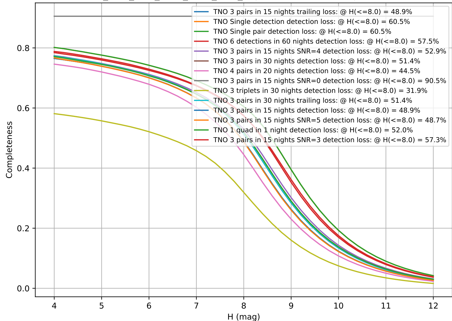
ddf_acor_sf15_lsf30_lsr20_v3.4_10yrs: CumulativeCompleteness
