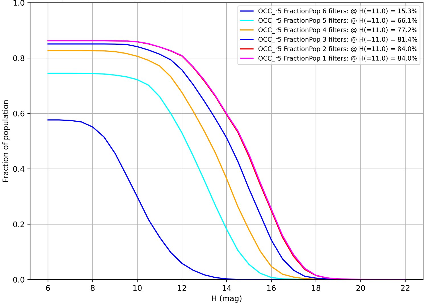
ddf_acor_sf15_lsf30_lsr20_v3.4_10yrs: Fraction of population with colors in X filters OCC_r5
