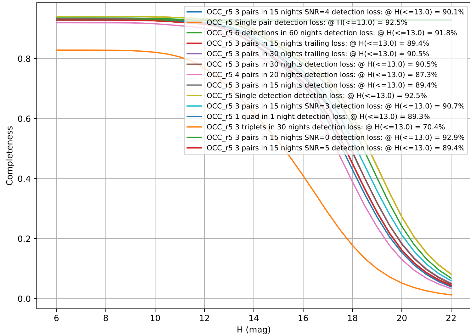
ddf_acor_sf15_lsf30_lsr20_v3.4_10yrs: CumulativeCompleteness
