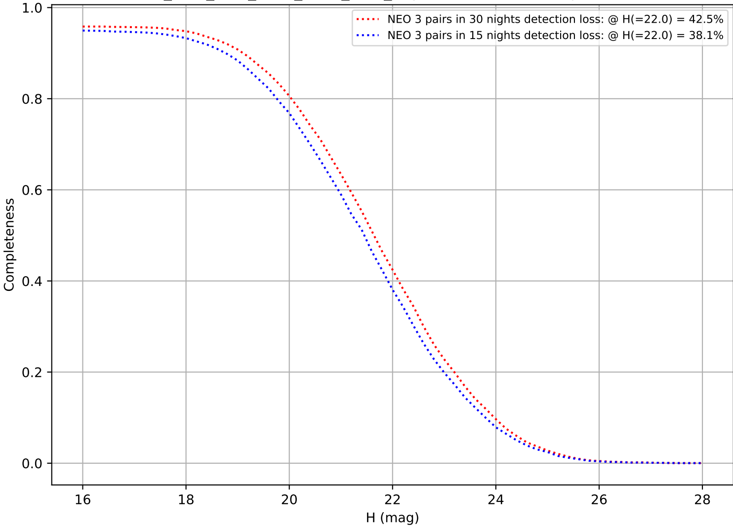
ddf_acor_sf15_lsf30_lsr20_v3.4_10yrs: DifferentialCompleteness
