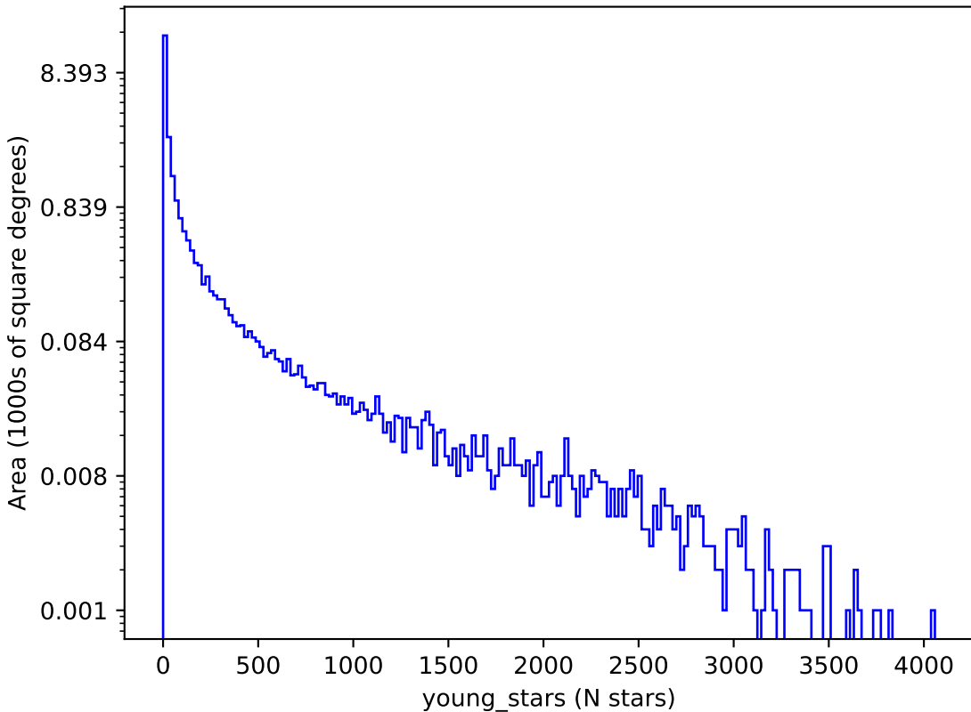
ddf_acor_sf15_lsf30_lsr20_v3.4_10yrs : young_stars
