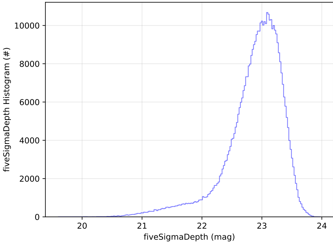
ddf_acor_sf15_lsf30_lsr20_v3.4_10yrs z: fiveSigmaDepth Histogram
