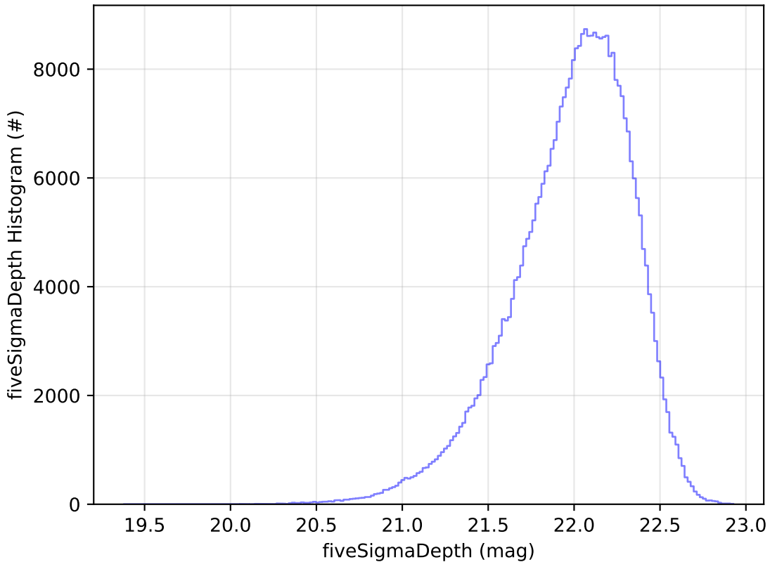
ddf_acor_sf15_lsf30_lsr20_v3.4_10yrs y: fiveSigmaDepth Histogram
