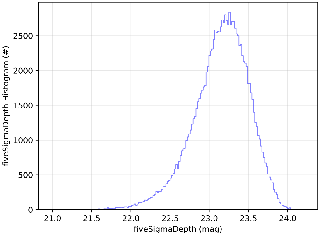
ddf_acor_sf15_lsf30_lsr20_v3.4_10yrs u: fiveSigmaDepth Histogram
