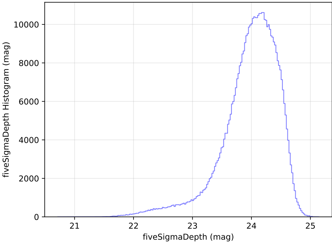
ddf_acor_sf15_lsf30_lsr20_v3.4_10yrs r: fiveSigmaDepth Histogram
