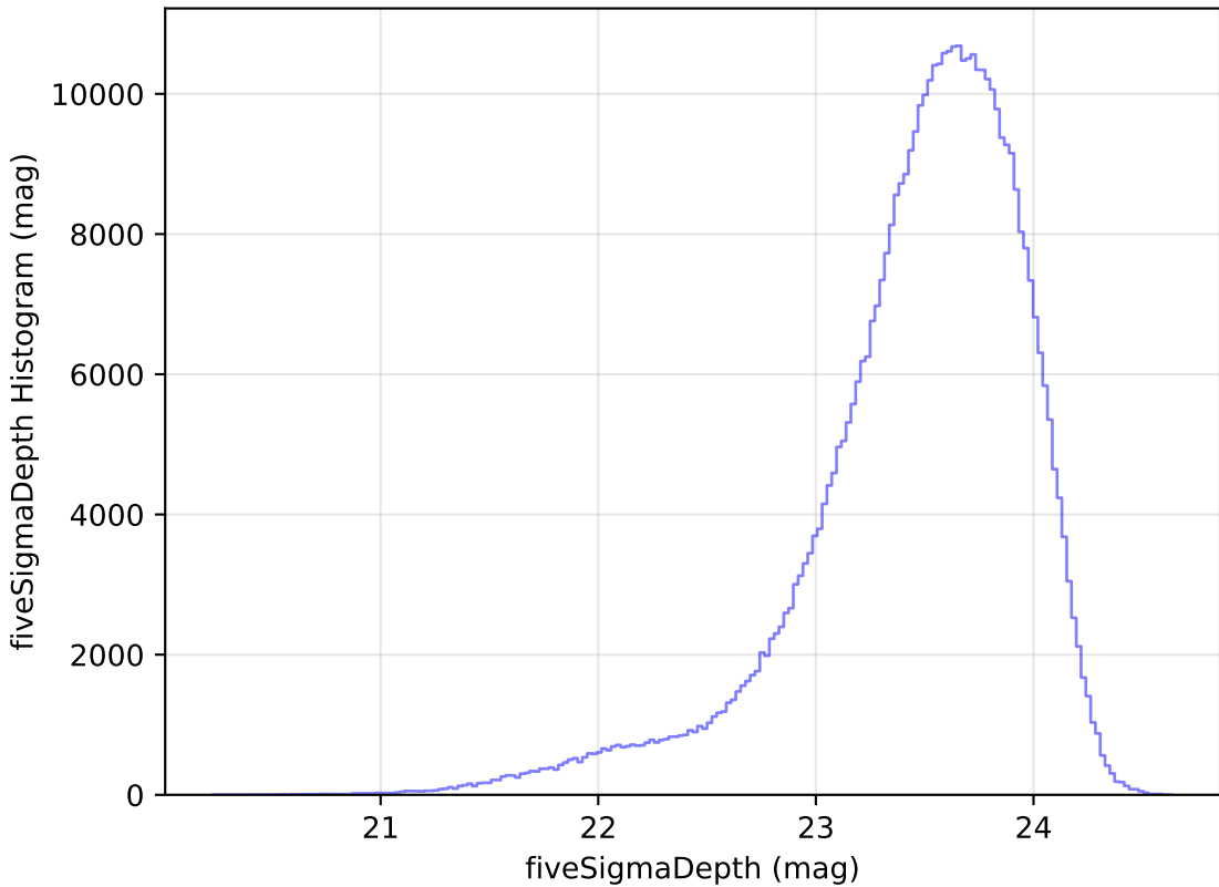
ddf_acor_sf15_lsf30_lsr20_v3.4_10yrs i: fiveSigmaDepth Histogram
