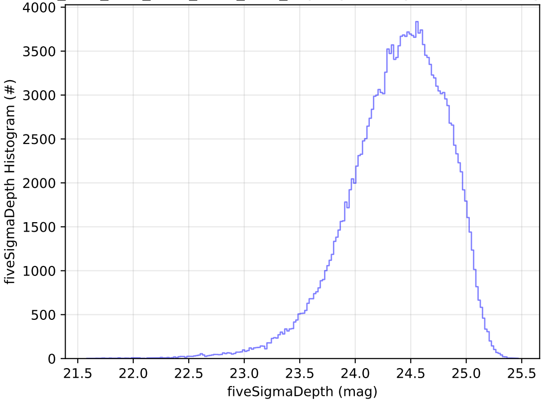
ddf_acor_sf15_lsf30_lsr20_v3.4_10yrs g: fiveSigmaDepth Histogram
