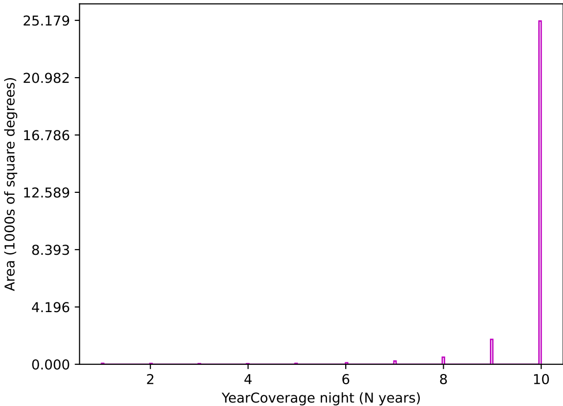
ddf_acor_sf15_lsf30_lsr20_v3.4_10yrs z band: YearCoverage night
