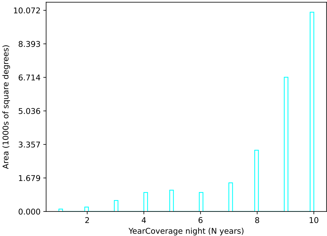
ddf_acor_sf15_lsf30_lsr20_v3.4_10yrs u band: YearCoverage night
