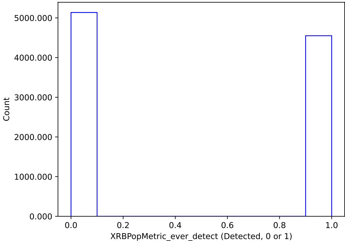
ddf_acor_sf15_lsf30_lsr20_v3.4_10yrs : XRBPoMetric_ever_detect
