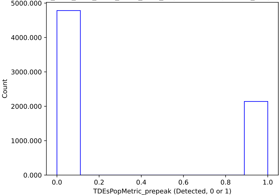
ddf_acor_sf15_lsf30_lsr20_v3.4_10yrs : TDEsPopMetric_prepeak
