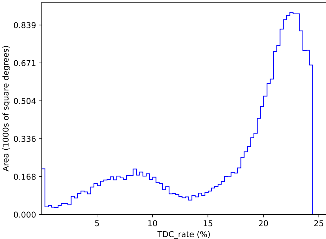
ddf_acor_sf15_lsf30_lsr20_v3.4_10yrs : TDC_rate
