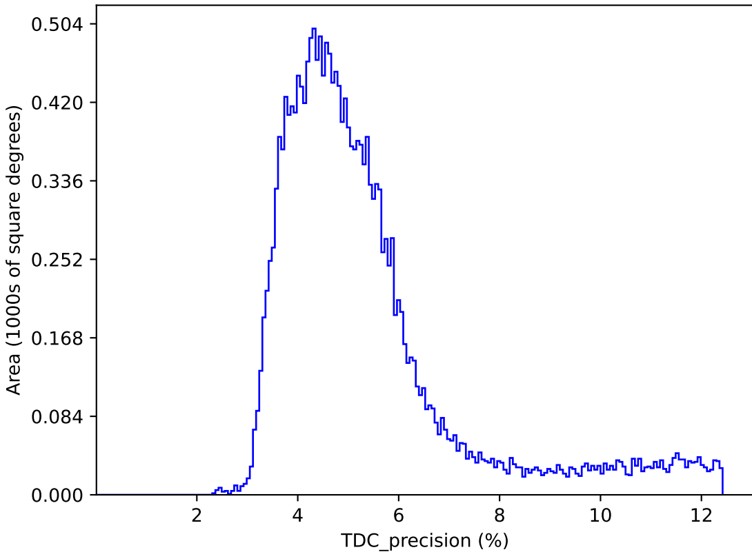
ddf_acor_sf15_lsf30_lsr20_v3.4_10yrs : TDC_precision
