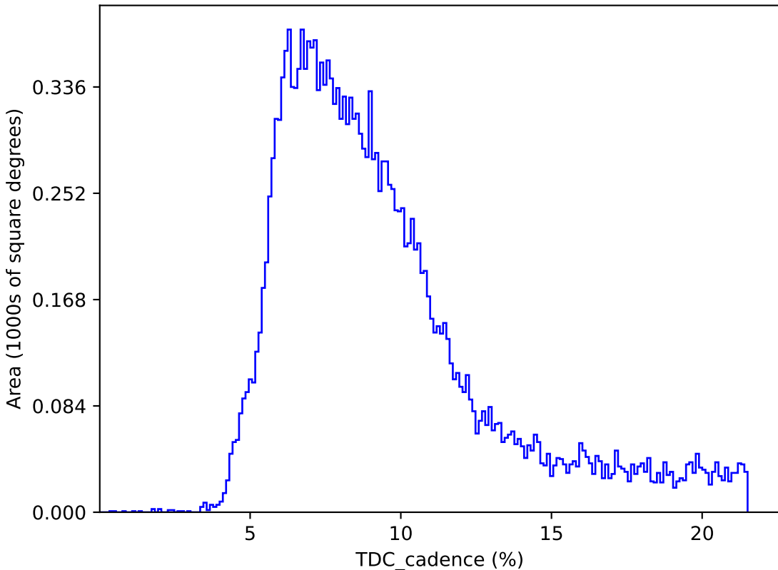
ddf_acor_sf15_ls30_lsr20_v3.4_10yrs : TDC_cadence
