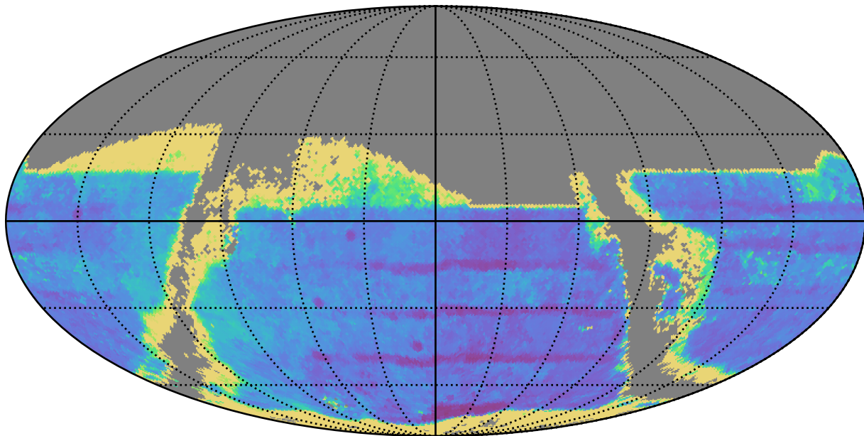
ddf_acor_sf15_lsf30_lsr20_v3.4_10yrs : TDC_accuracy
