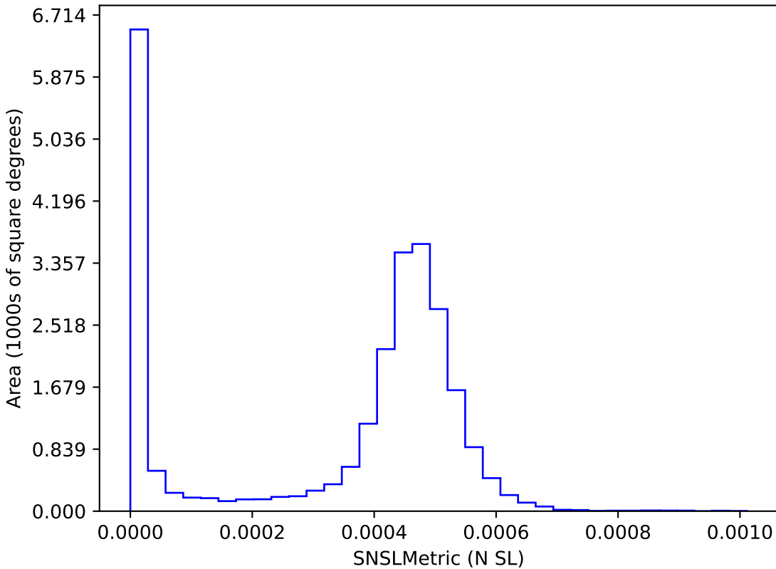
ddf_acor_sf15_lsf30_lsr20_v3.4_10yrs : SNSLMetric
