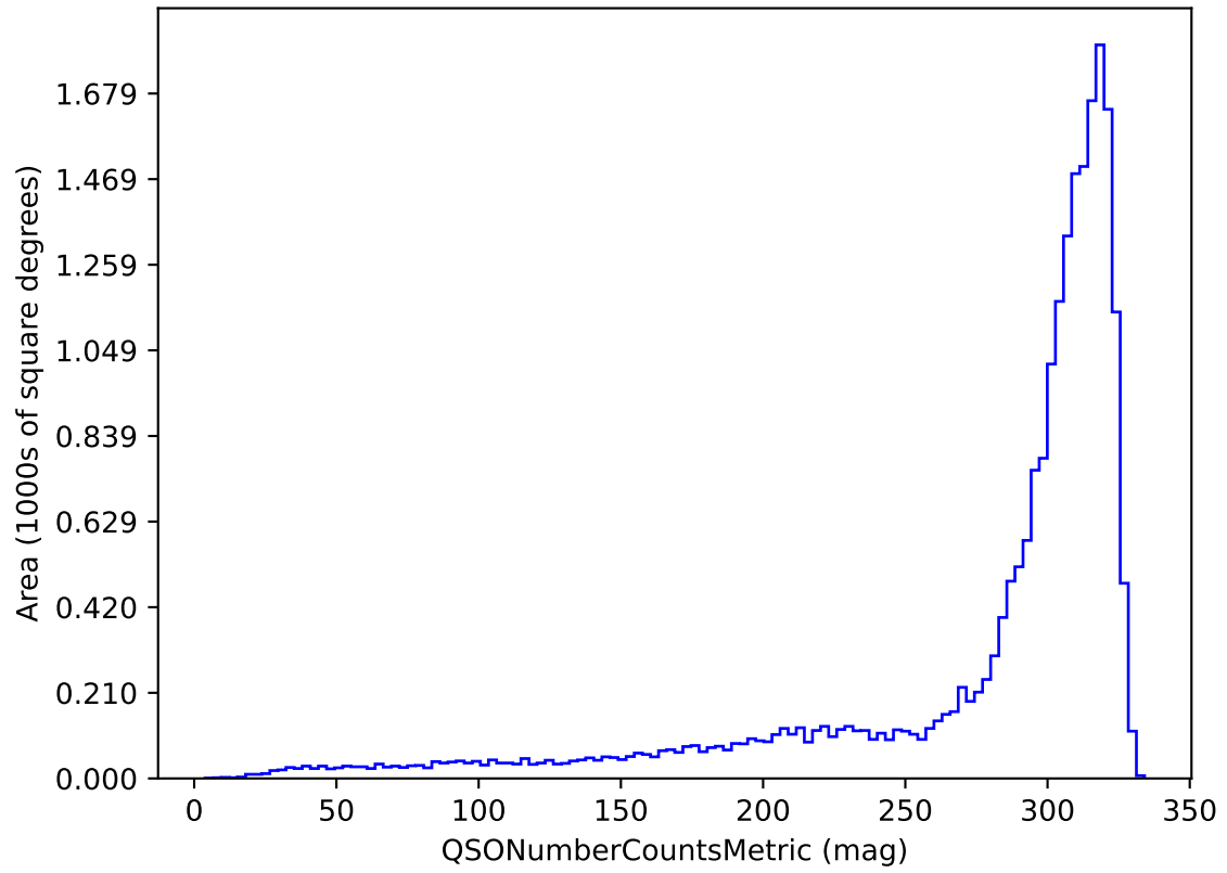
ddf_acor_sf15_lsf30_lsr20_v3.4_10yrs u band and non-DD: QSONumberCountsMetric
