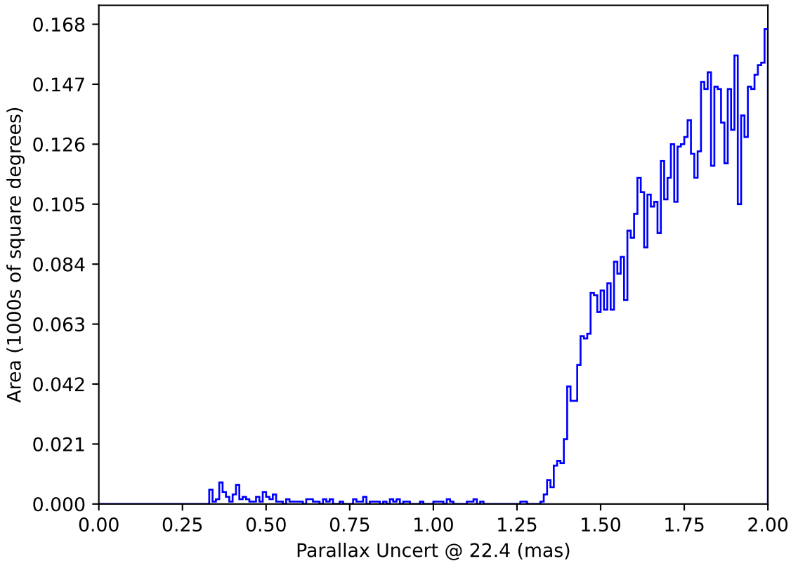
ddf_acor_sf15_lsf30_lsr20_v3.4_10yrs : Parallax Uncert @ 22.4
