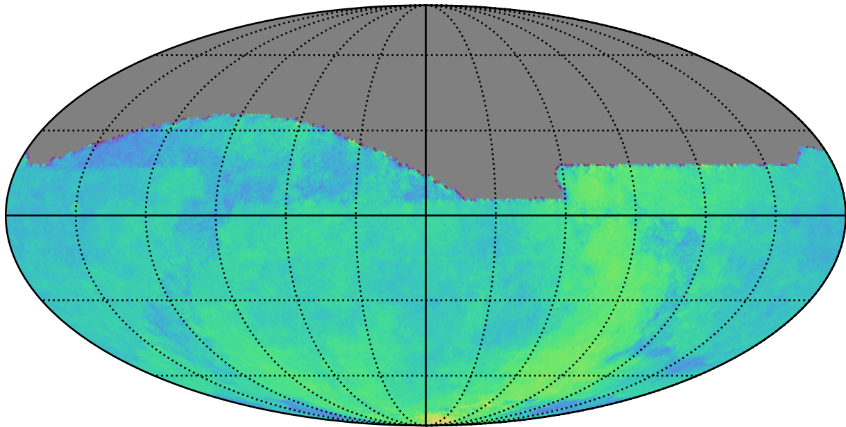
ddf_acor_sf15_lsf30_lsr20_v3.4_10yrs : Parallax Coverage @ 24.0
