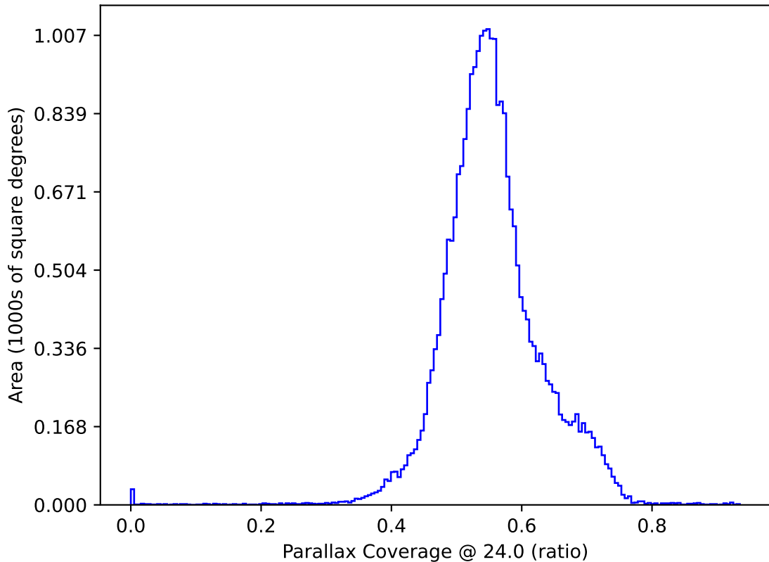
ddf_acor_sf15_lsf30_lsr20_v3.4_10yrs : Parallax Coverage @ 24.0
