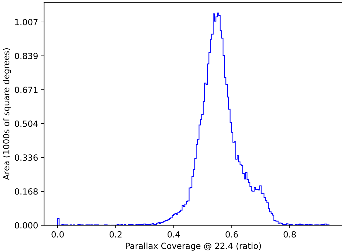
ddf_acor_sf15_lsf30_lsr20_v3.4_10yrs : Parallax Coverage @ 22.4
