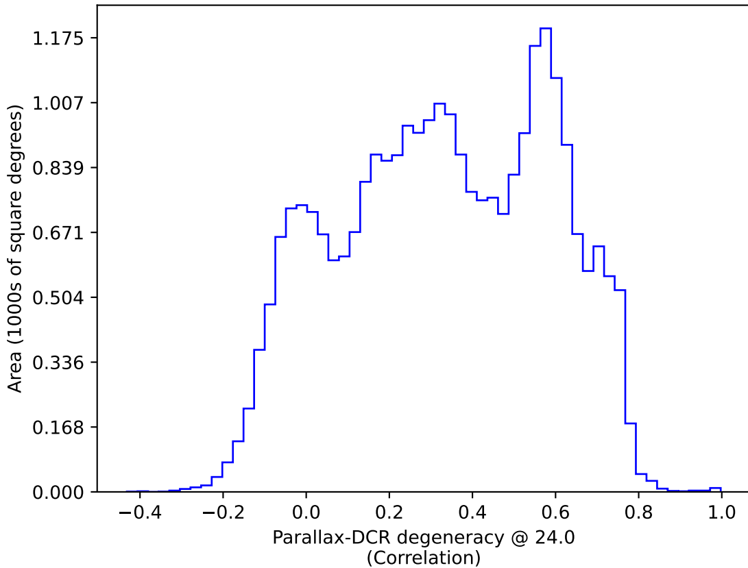
ddf_acor_sf15_lsf30_lsr20_v3.4_10yrs : Parallax-DCR degeneracy @ 24.0
