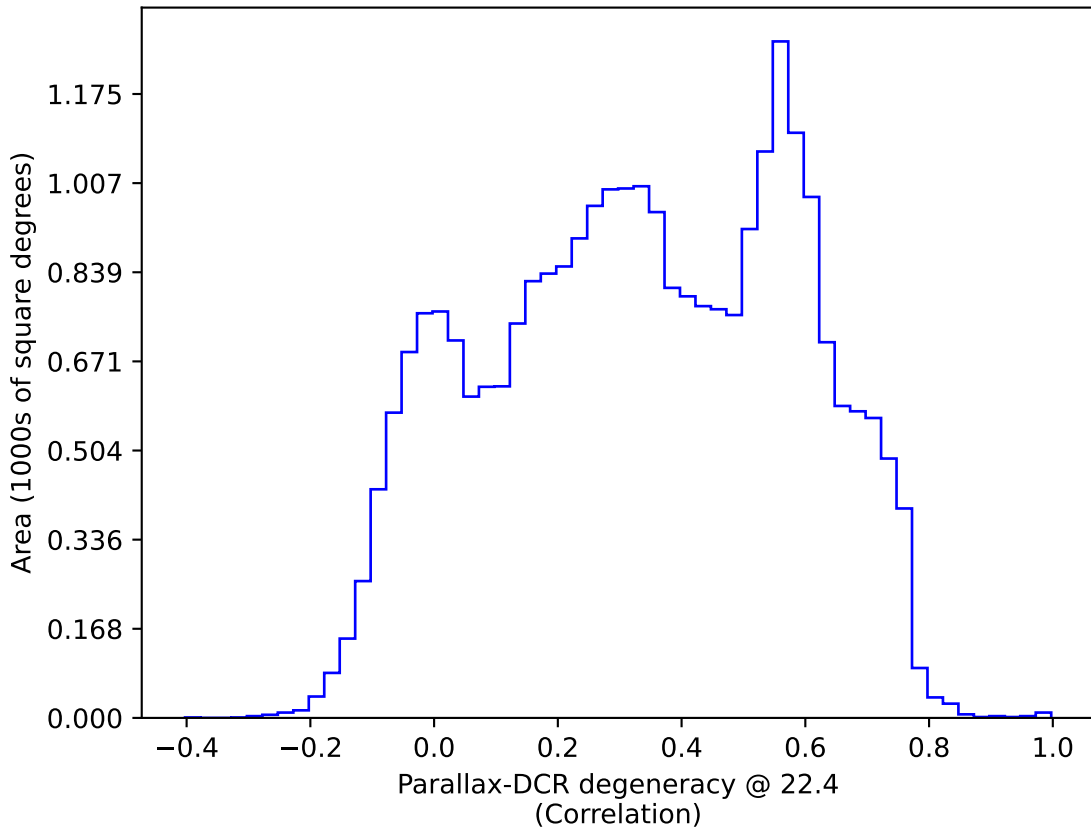
ddf_acor_sf15_lsf30_lsr20_v3.4_10yrs : Parallax-DCR degeneracy @ 22.4
