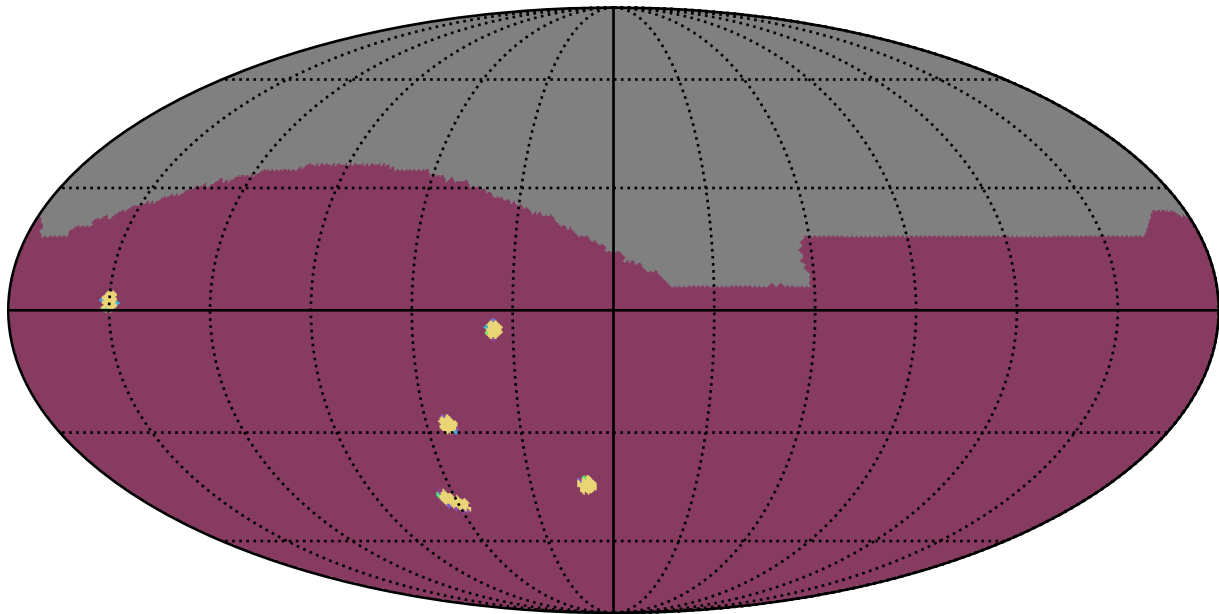
ddf_acor_sf15_lsf30_lsr20_v3.4_10yrs : NumberOfQuickRevisits
