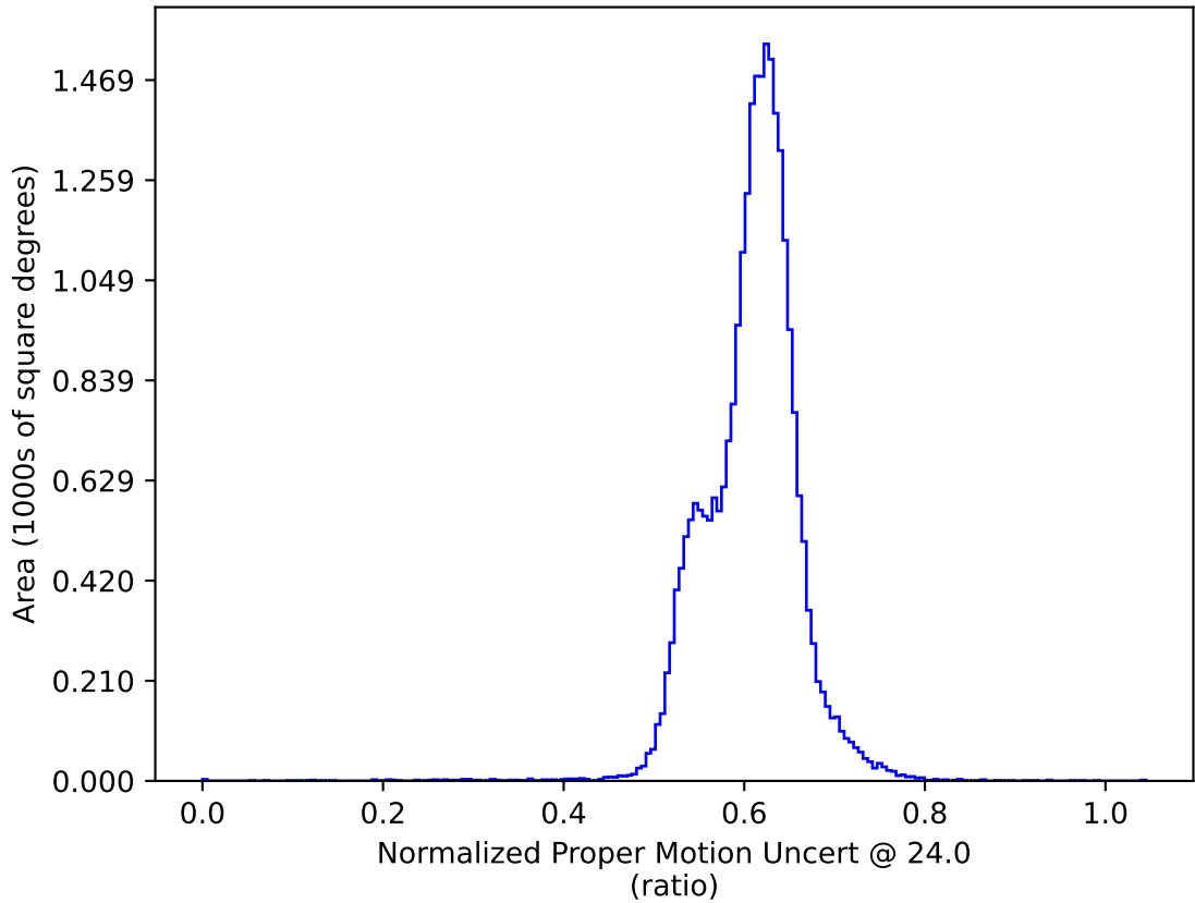
ddf_acor_sf15_lsf30_lsr20_v3.4_10yrs : Normalized Proper Motion Uncert @ 24.0
