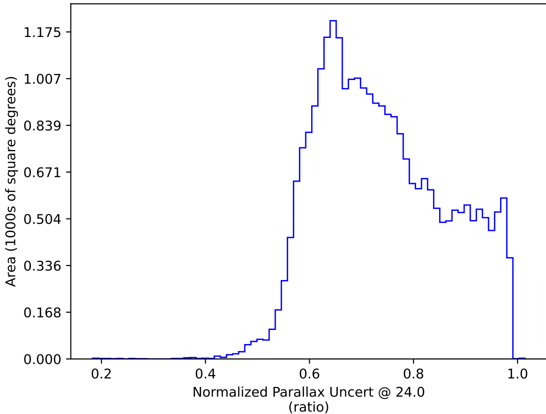
ddf_acor_sf15_lsf30_lsr20_v3.4_10yrs : Normalized Parallax Uncert @ 24.0
