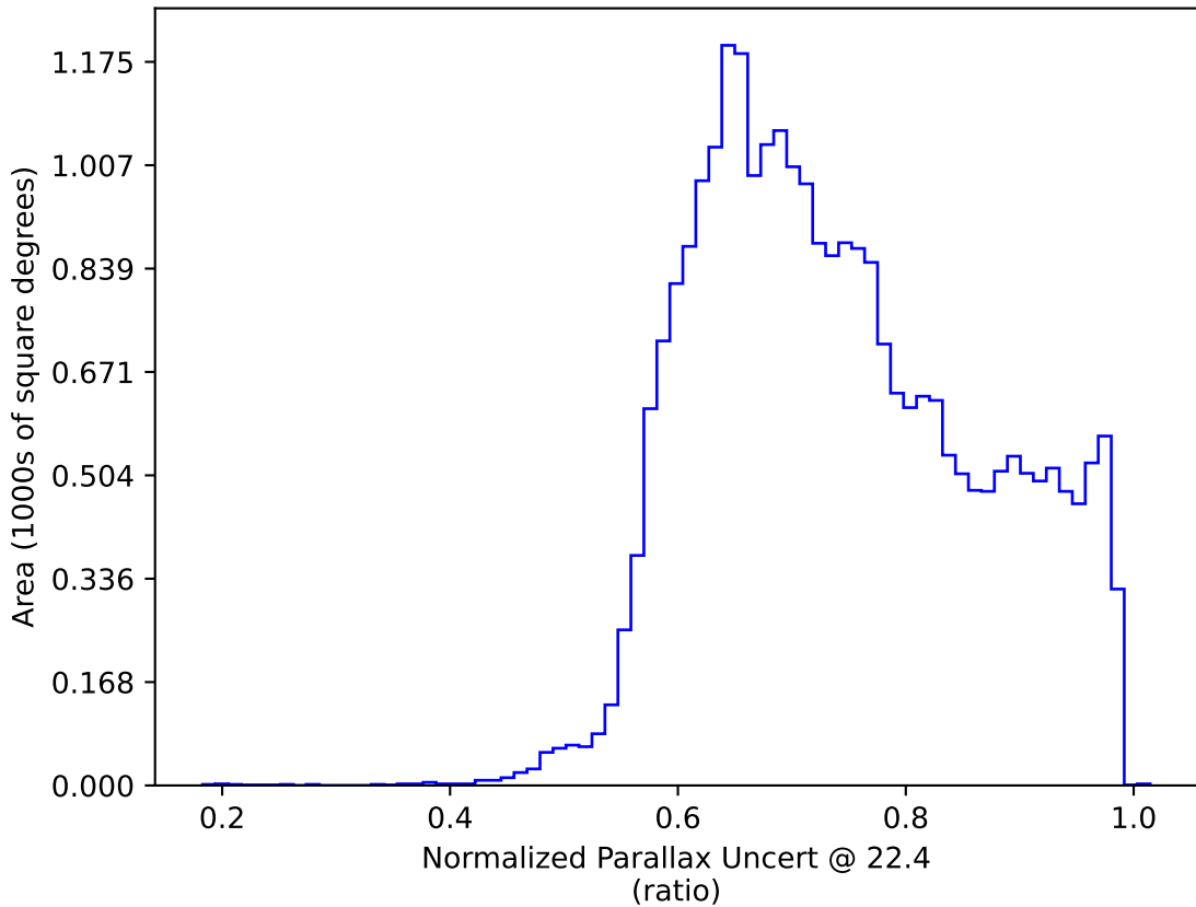
ddf_acor_sf15_lsf30_lsr20_v3.4_10yrs : Normalized Parallax Uncert @ 22.4
