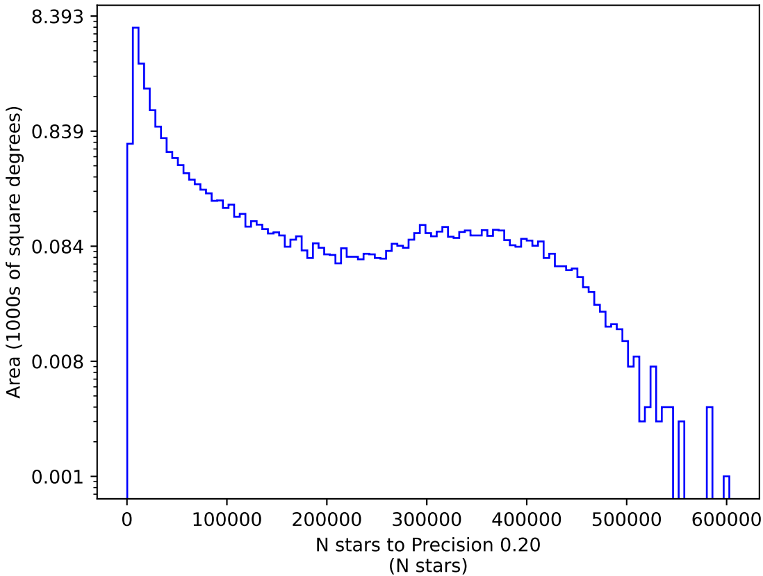
ddf_acor_sf15_lsf30_lsr20_v3.4_10yrs y: N stars to Precision 0.20
