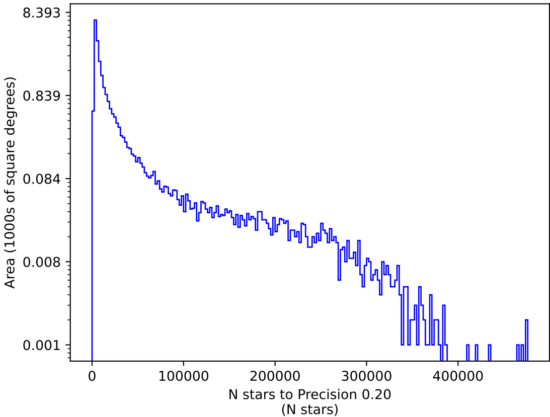
ddf_acor_sf15_ls30_lsr20_v3.4_10yrs u: N stars to Precision 0.20
