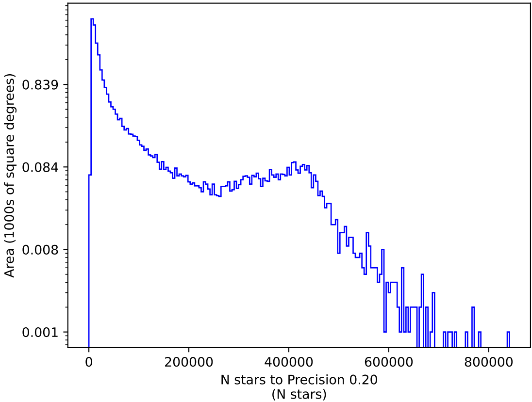
ddf_acor_sf15_lsf30_lsr20_v3.4_10yrs r: N stars to Precision 0.20
