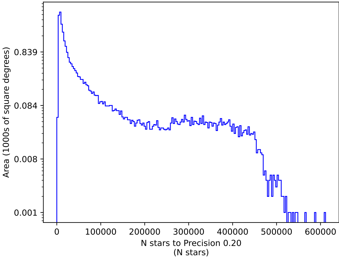
ddf_acor_sf15_lsf30_lsr20_v3.4_10yrs g: N stars to Precision 0.20
