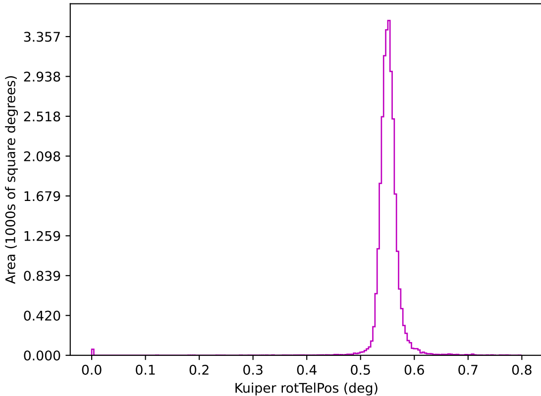
ddf_acor_sf15_lsf30_lsr20_v3.4_10yrs z: Kuiper rotTelPos
