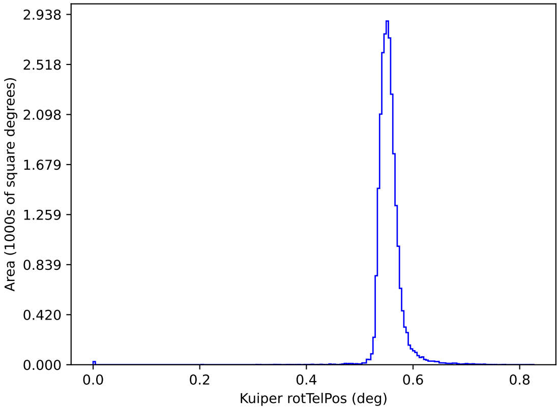
ddf_acor_sf15_lsf30_lsr20_v3.4_10yrs y: Kuiper rotTelPos
