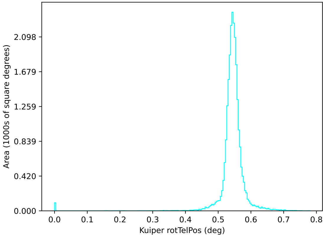
ddf_acor_sf15_ls30_lsr20_v3.4_10yrs u: Kuiper rotTelPos
