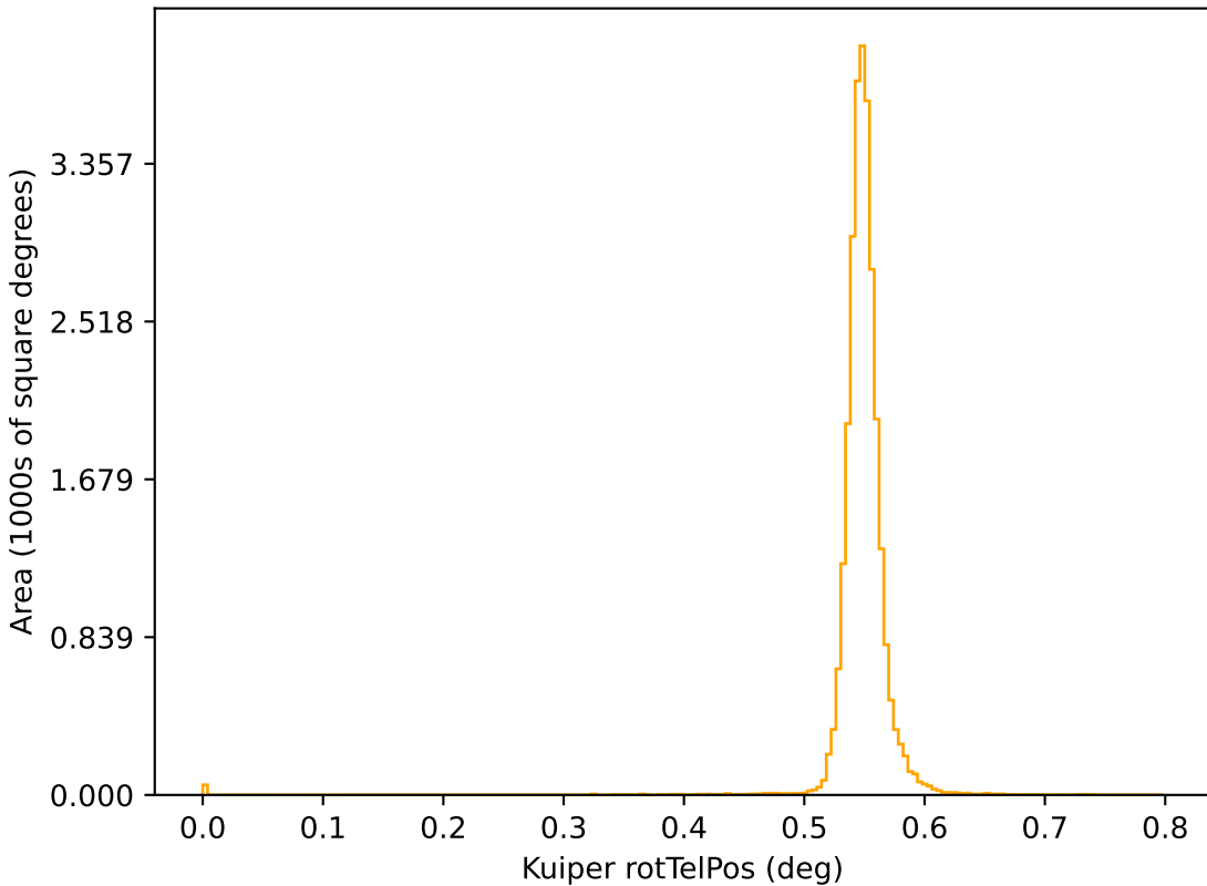
ddf_acor_sf15_lsf30_lsr20_v3.4_10yrs r: Kuiper rotTelPos
