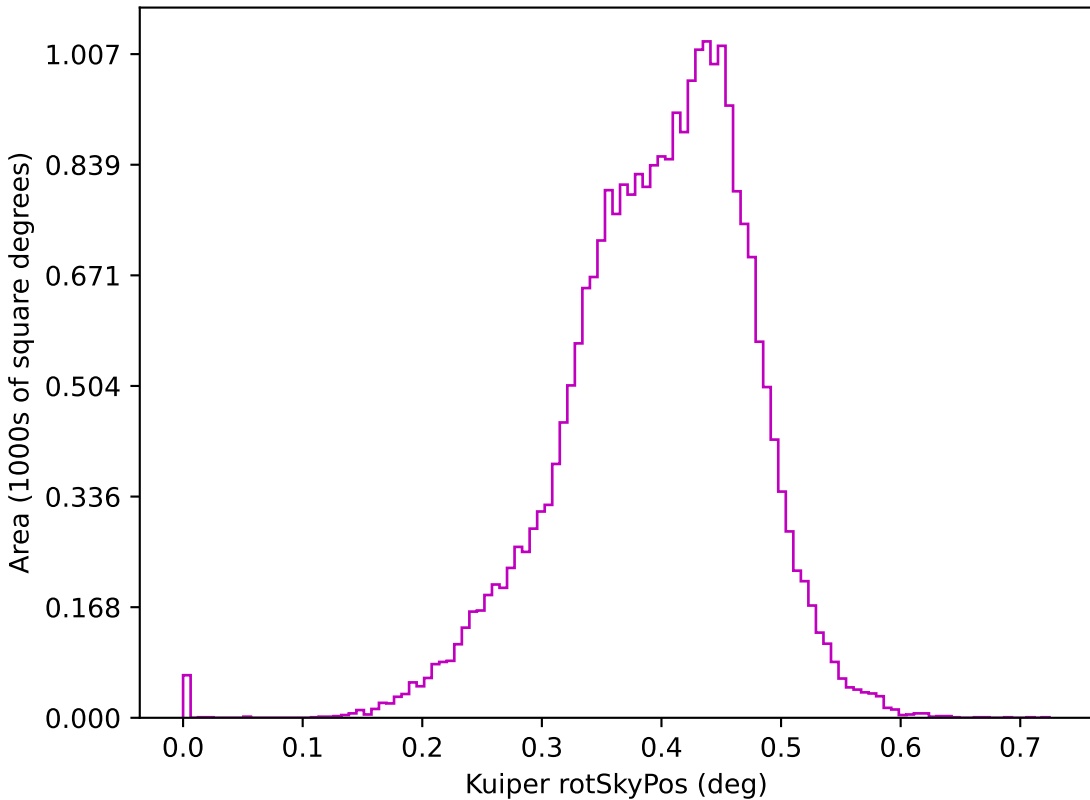
ddf_acor_sf15_lsf30_lsr20_v3.4_10yrs z: Kuiper rotSkyPos
