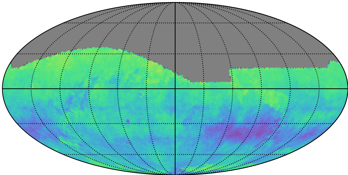
ddf_acor_sf15_lsf30_lsr20_v3.4_10yrs r: Kuiper rotSkyPos
