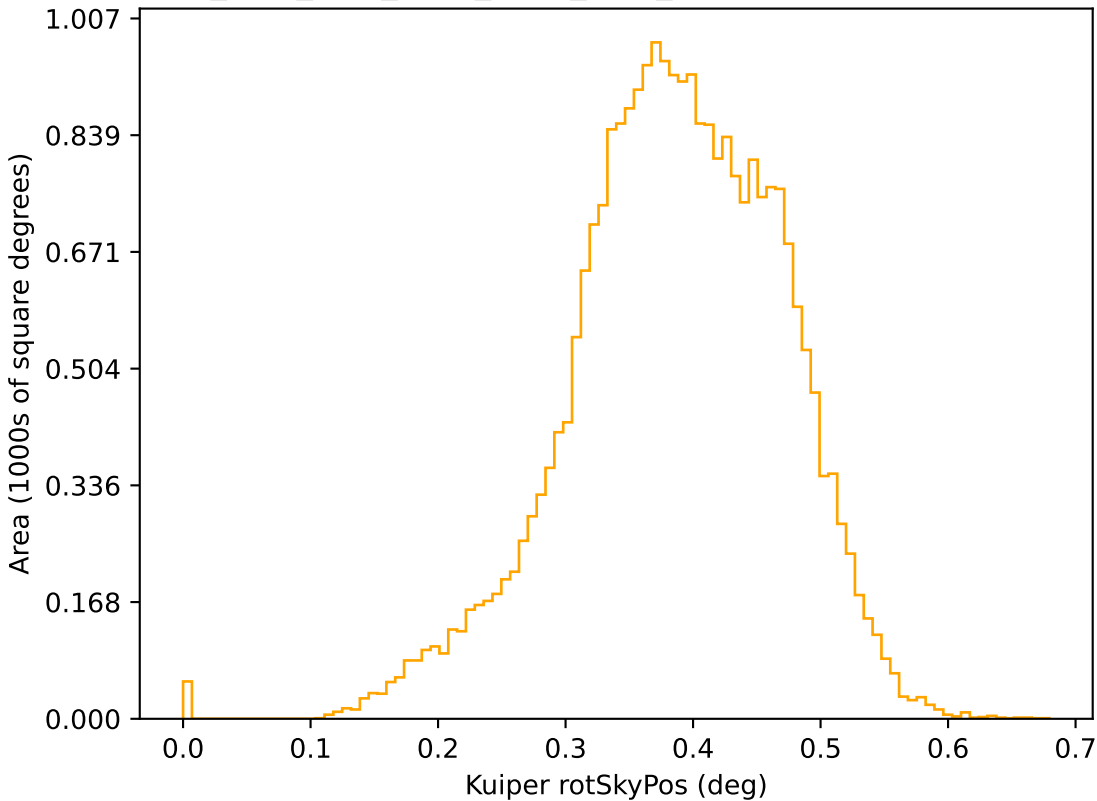
ddf_acor_sf15_lsf30_lsr20_v3.4_10yrs r: Kuiper rotSkyPos
