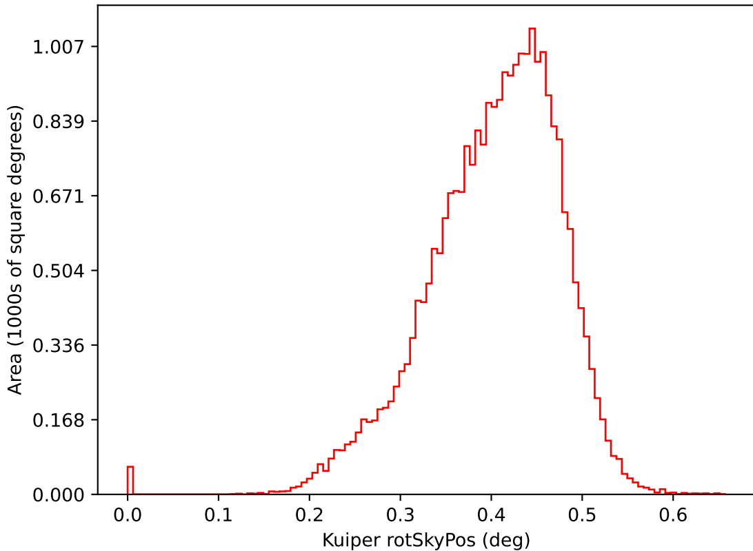
ddf_acor_sf15_ls30_lsr20_v3.4_10yrs i: Kuiper rotSkyPos
