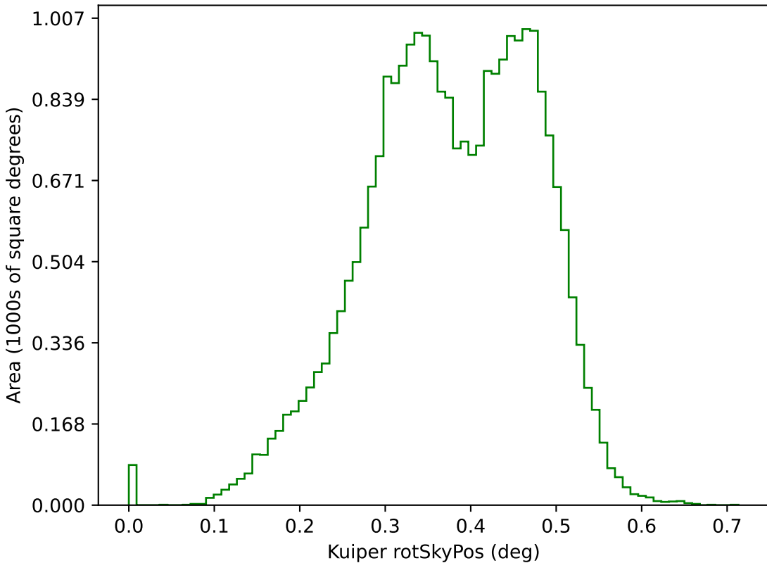
ddf_acor_sf15_lsf30_lsr20_v3.4_10yrs g: Kuiper rotSkyPos
