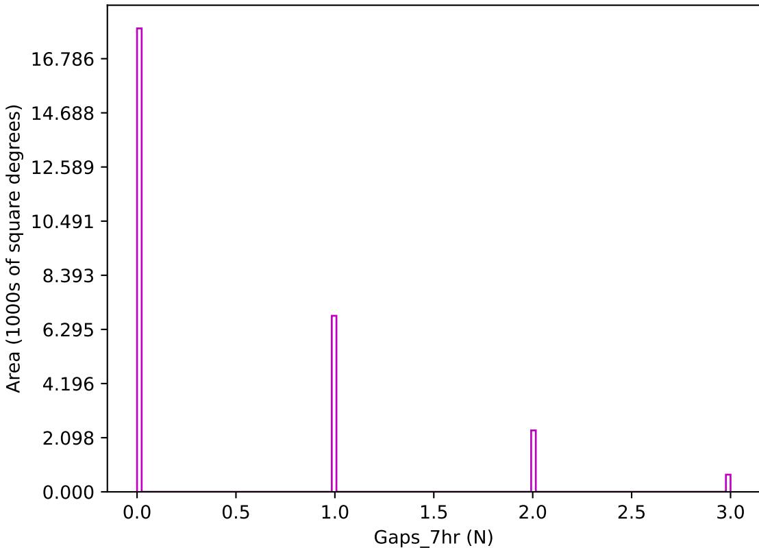
ddf_acor_sf15_ls30_lsr20_v3.4_10yrs z band: Gaps_7hr
