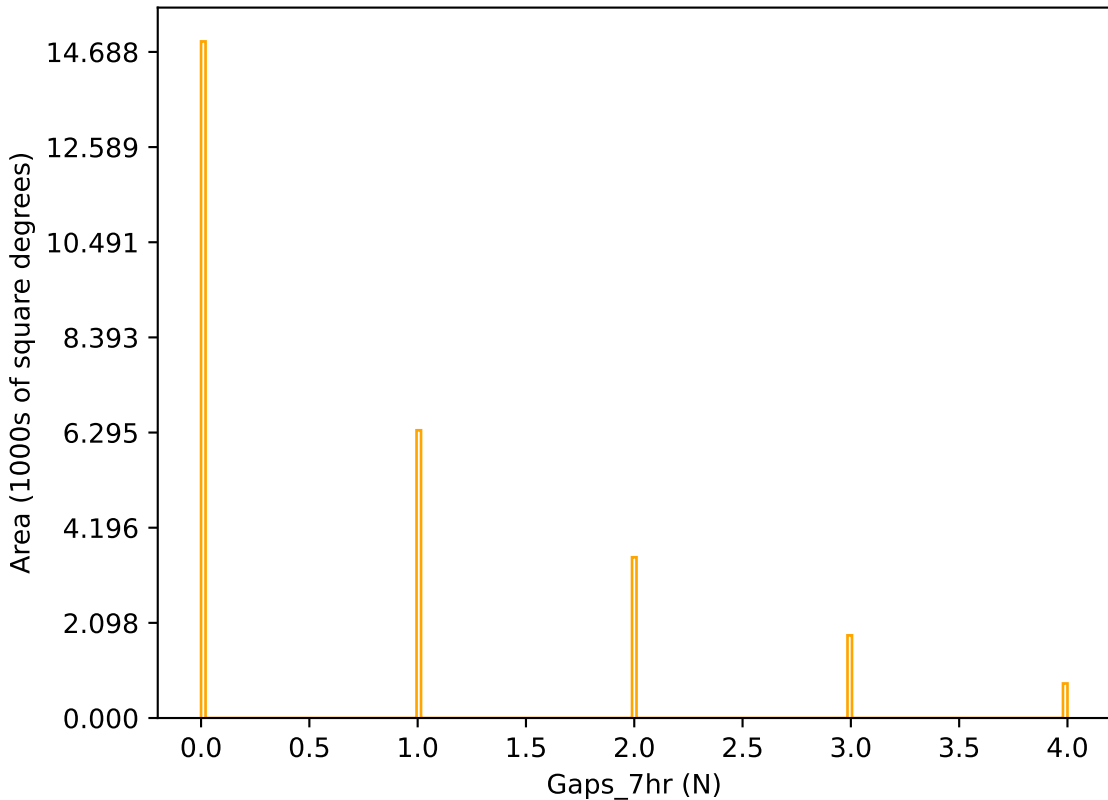
ddf_acor_sf15_lsf30_lsr20_v3.4_10yrs r band: Gaps_7hr
