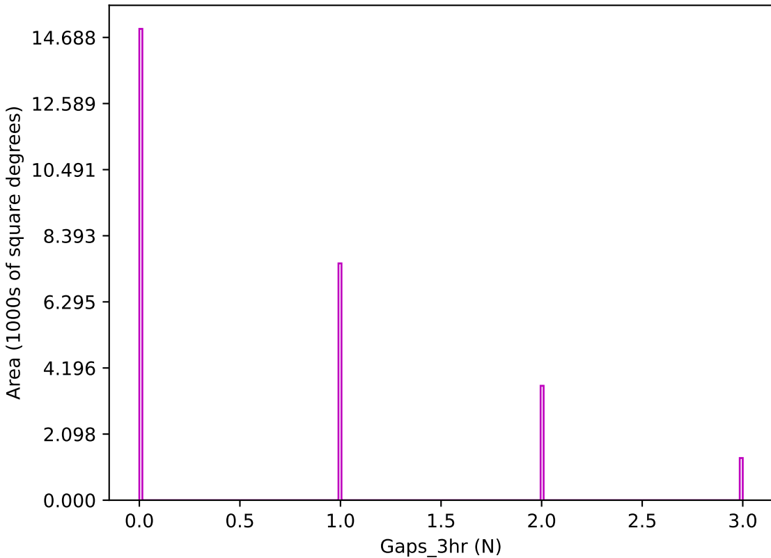
ddf_acor_sf15_ls30_lsr20_v3.4_10yrs z band: Gaps_3hr
