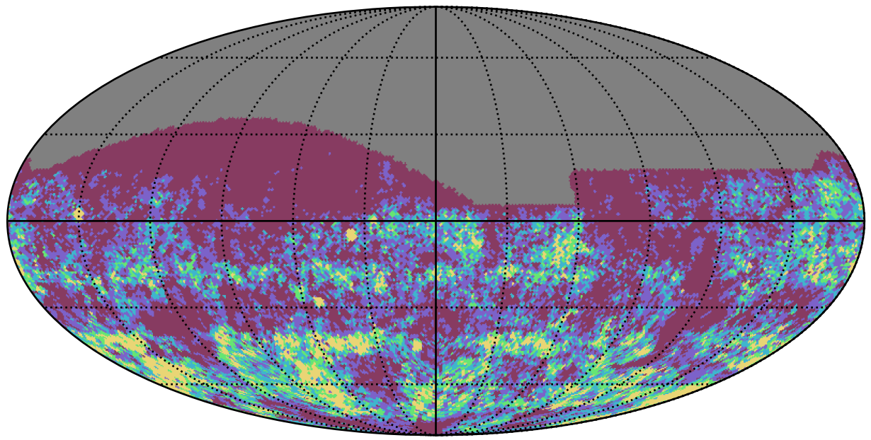
ddf_acor_sf15_lsf30_lsr20_v3.4_10yrs r band: Gaps_3hr
